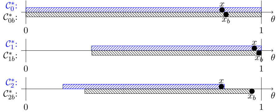
Figure 7: Example 1 with constant bias b = \frac{1}{3} on top and with state-dependent bias, b(\theta) = \frac{1}{3} + \frac{1}{30}\theta below: the obligatorily complete contracts, 1-step optimal contracts, and the 2-step optimal contracts.
