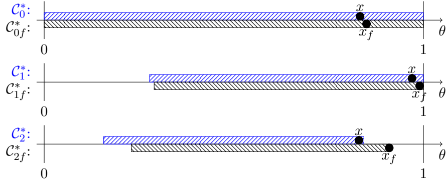
Figure 8: Example 1 with uniform distribution on top and with distribution, f(\theta) = \frac{9}{10} + \frac{2}{10}\theta below: the obligatorily complete contracts, 1-step optimal contracts, and the 2-step optimal contracts.
