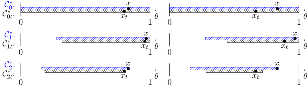
Figure 9: Example 1 with transfers, b = \frac{1}{3} , \alpha = 0.1 left panel and \alpha = 0.5 right panel: the obligatorily complete contracts, 1-step optimal contracts, and the 2-step optimal contracts.
