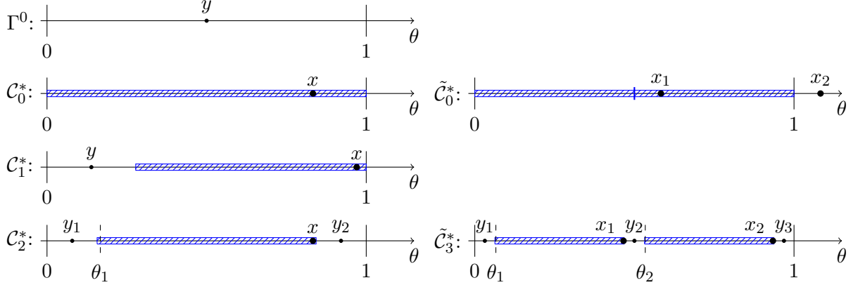
Figure 1: Left: the four candidates for optimal contracts, with \widehat{K} = 1 and b = \frac{1}{3} : \Gamma^0, \mathcal{C}_0^*, \mathcal{C}_1^*, \mathcal{C}_2^* . Right: two candidates for optimal contracts with \widehat{K} = 2 : obligatorily complete \tilde{\mathcal{C}}_0^* for b = \frac{1}{3} , and 3-step \tilde{\mathcal{C}}_3^* for b = \frac{1}{5} .
