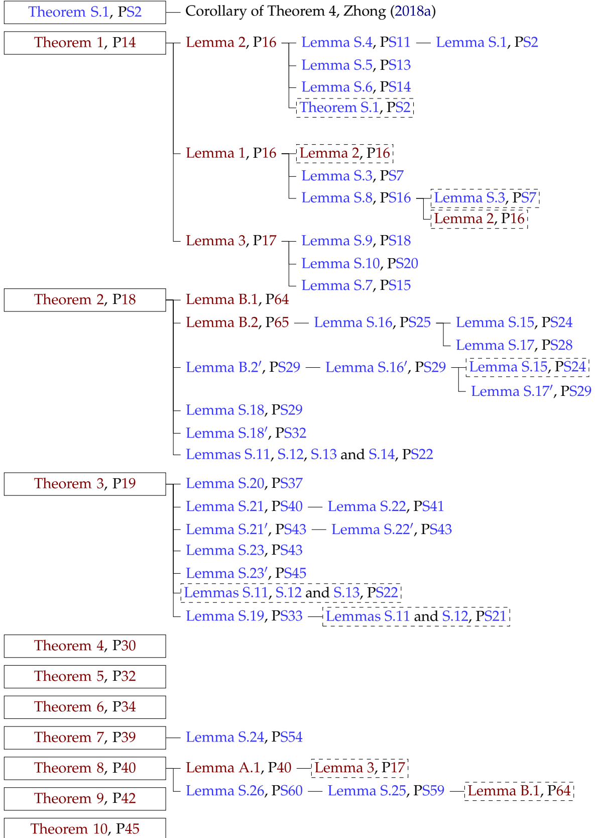
Figure 17: Roadmap for proofs
