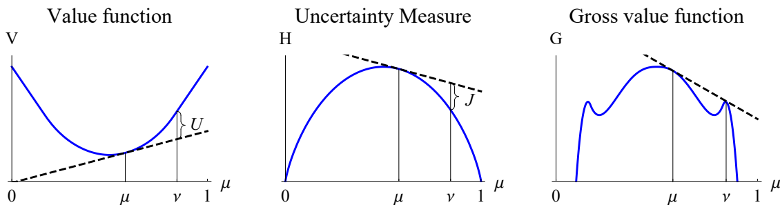
Figure 9: Concavification of the gross value function
