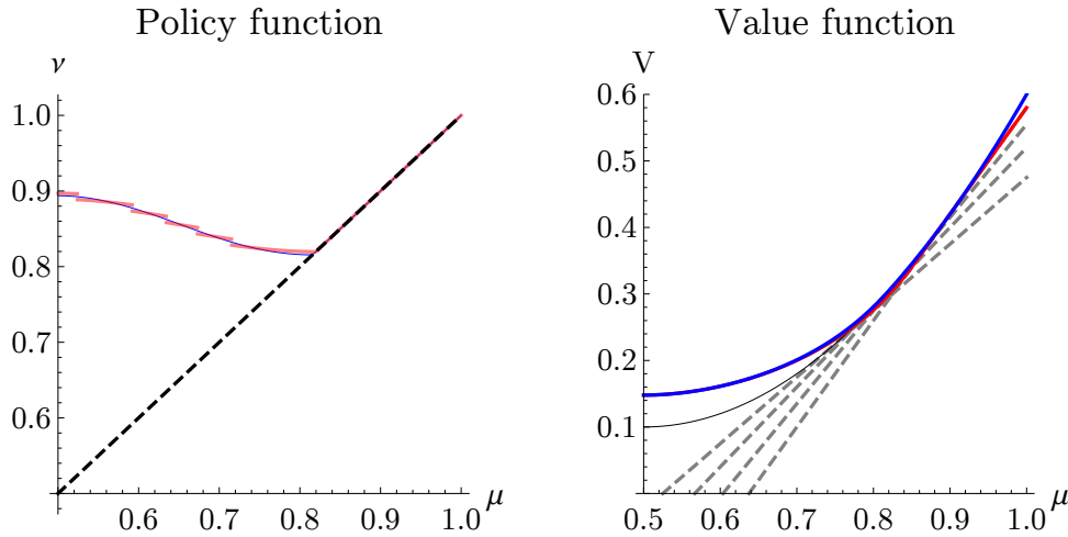
Left panel shows the optimal policy function with finite actions (red) and continuous actions (blue). The dashed line is \nu = \mu . Right panel shows the optimal value function. The thin black line is value from immediate action F(\mu) , the dashed lines are discrete approximations of the continuous function F .
