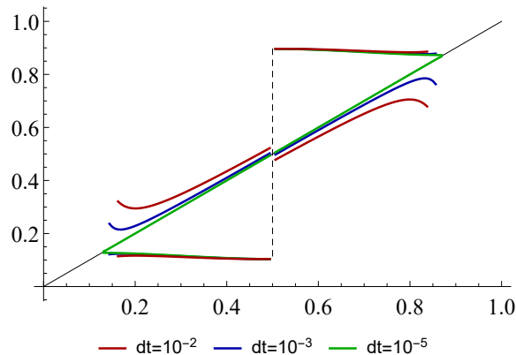
Figure 13: Convergence of policy function
