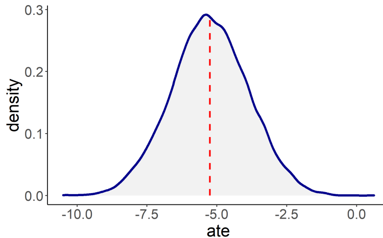
Figure 4: Academic achievement data: Posterior density of the ATE from model in which the effect of z_4 is non-parametric. Red dashed line is at -5.251, the posterior mean. Posterior density based on 20,000 posterior draws after 1,000 burn-in.
