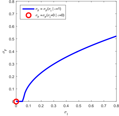
Figure 5: Best response function for firm in the final-goods sector
